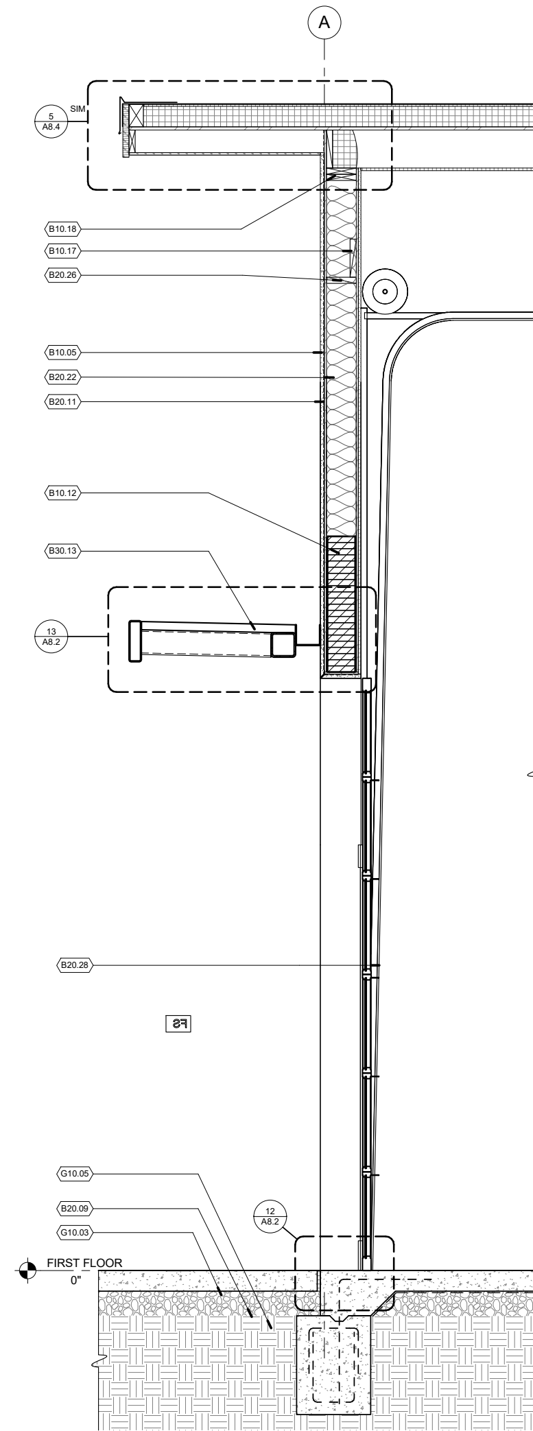
3 WALL SECTION @ ROLLING DOOR A3.5 3/4" = 1'-0"
