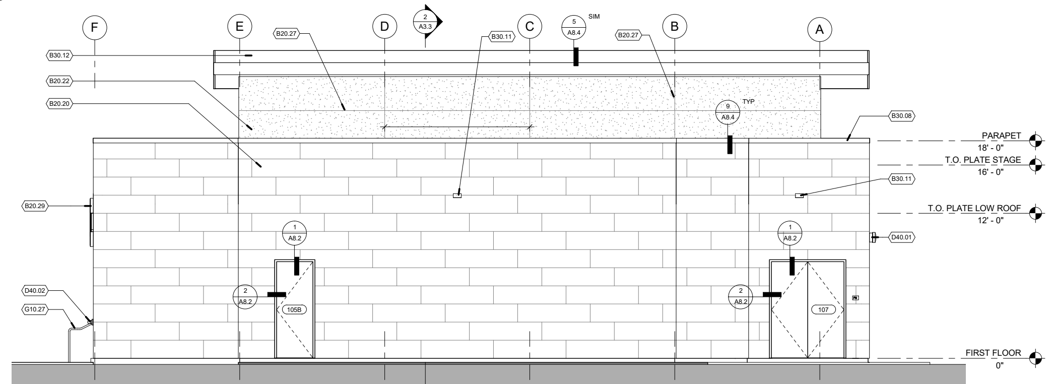
2 A3.2 EAST ELEVATION 1/4" = 1'-0"
