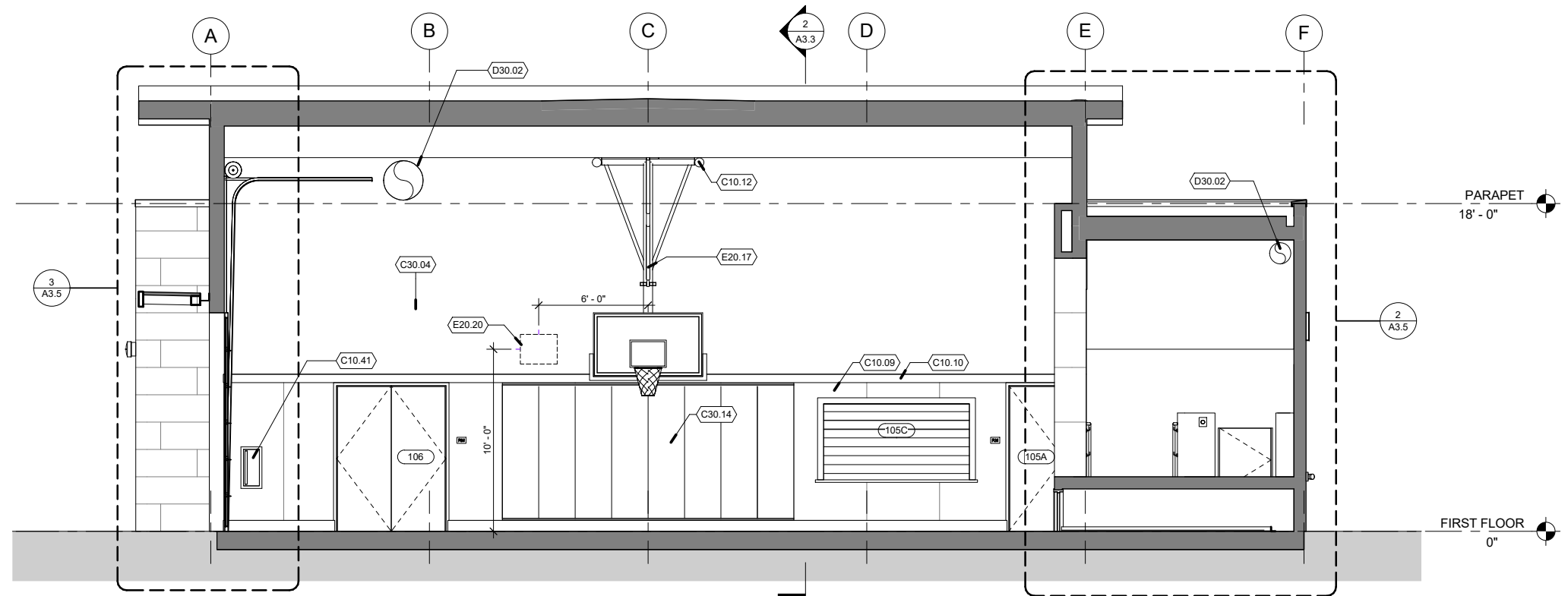
1 NORTH SOUTH BUILDING SECTION - STAGE & MULTIPURPOSE ROOM A3.3 1/4" = 1'-0"
