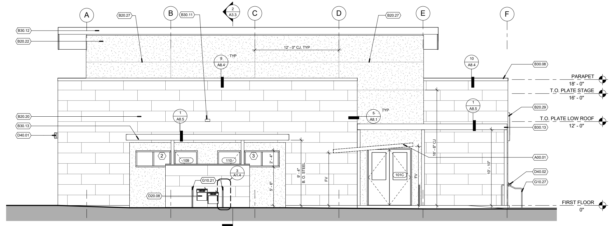
1 A3.2 WEST ELEVATION 1/4" = 1'-0"
