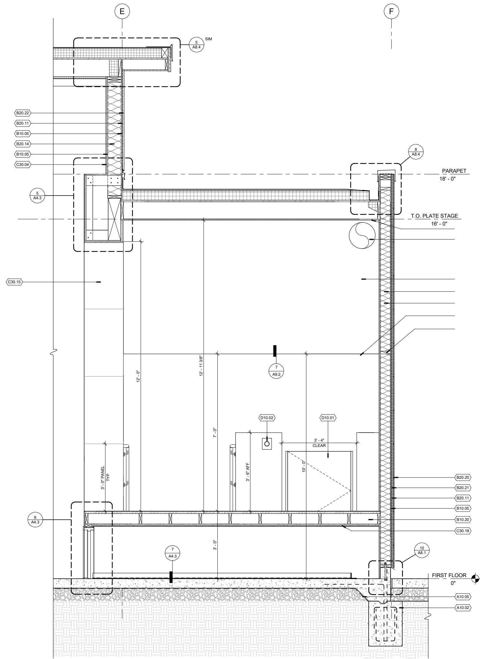
2 WALL SECTION THROUGH STAGE A3.5 3/4" = 1'-0"
