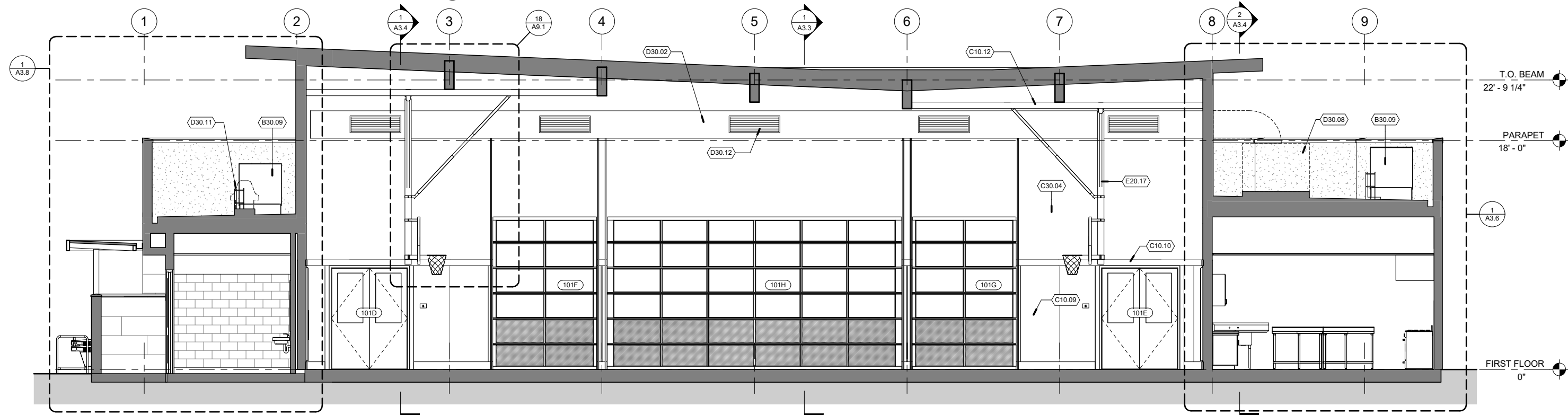
2 EAST WEST BUILDING SECTION A3.3 1/4" = 1'-0"
